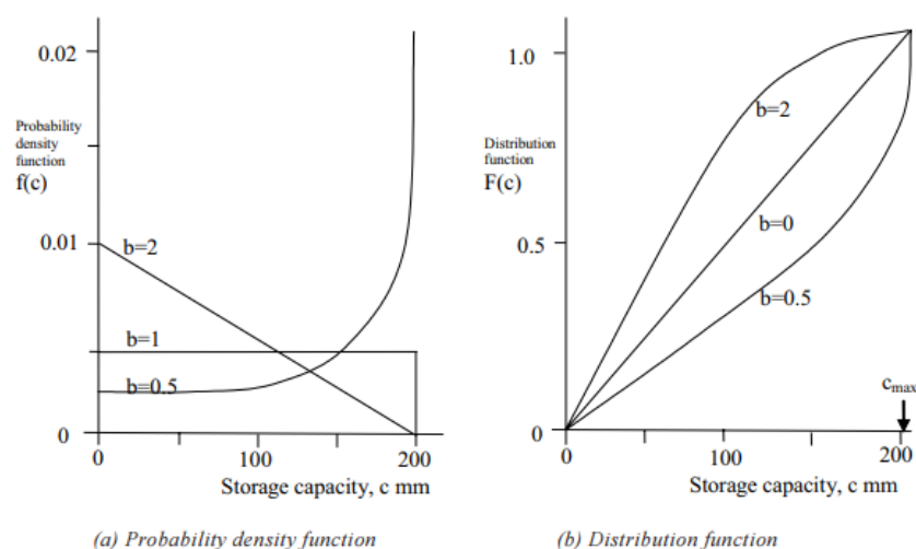
Figure 5. The Pareto distribution after Moore, 2007.
