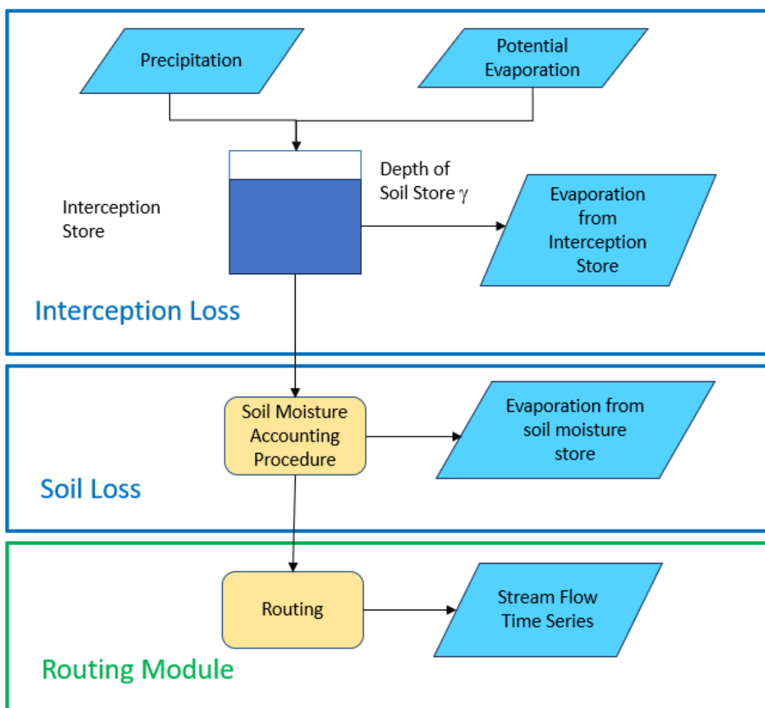
Figure 3. The interception sub-module within CERF.
