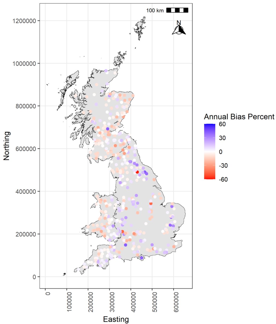
Figure 13. Spatial distribution of the Annual Bias for the CERF2-HadUK development dataset.
