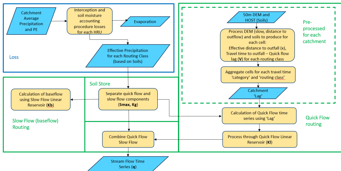
Figure 6. Flowchart of CERF semi-distributed model structure, highlighting the routing module.
