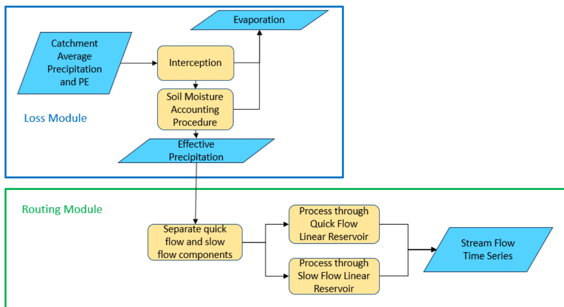
Figure 1. The CERF structure illustrating the loss module and the routing module.
