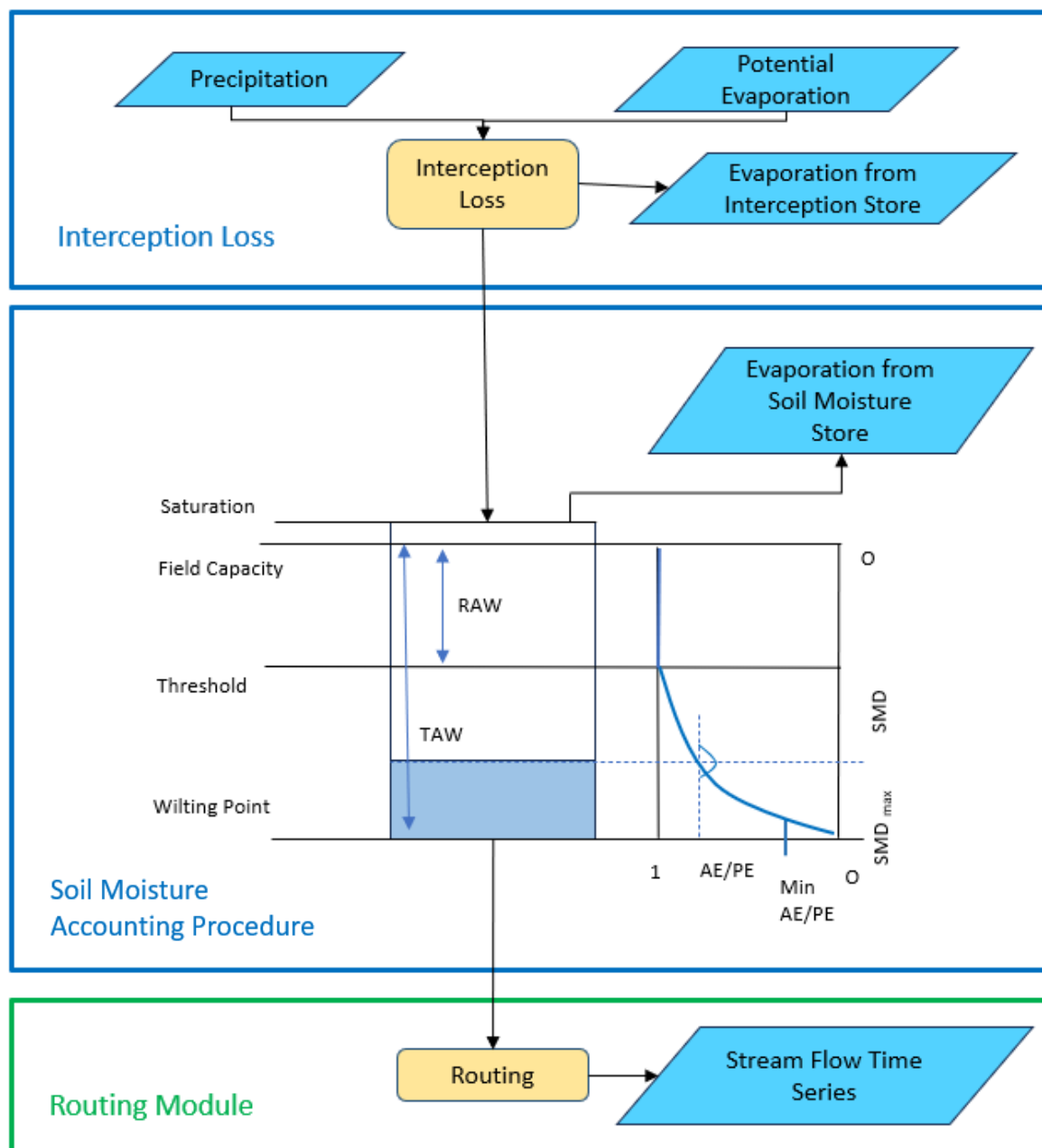
Figure 4. The soil moisture accounting procedure sub-module within CERF.
