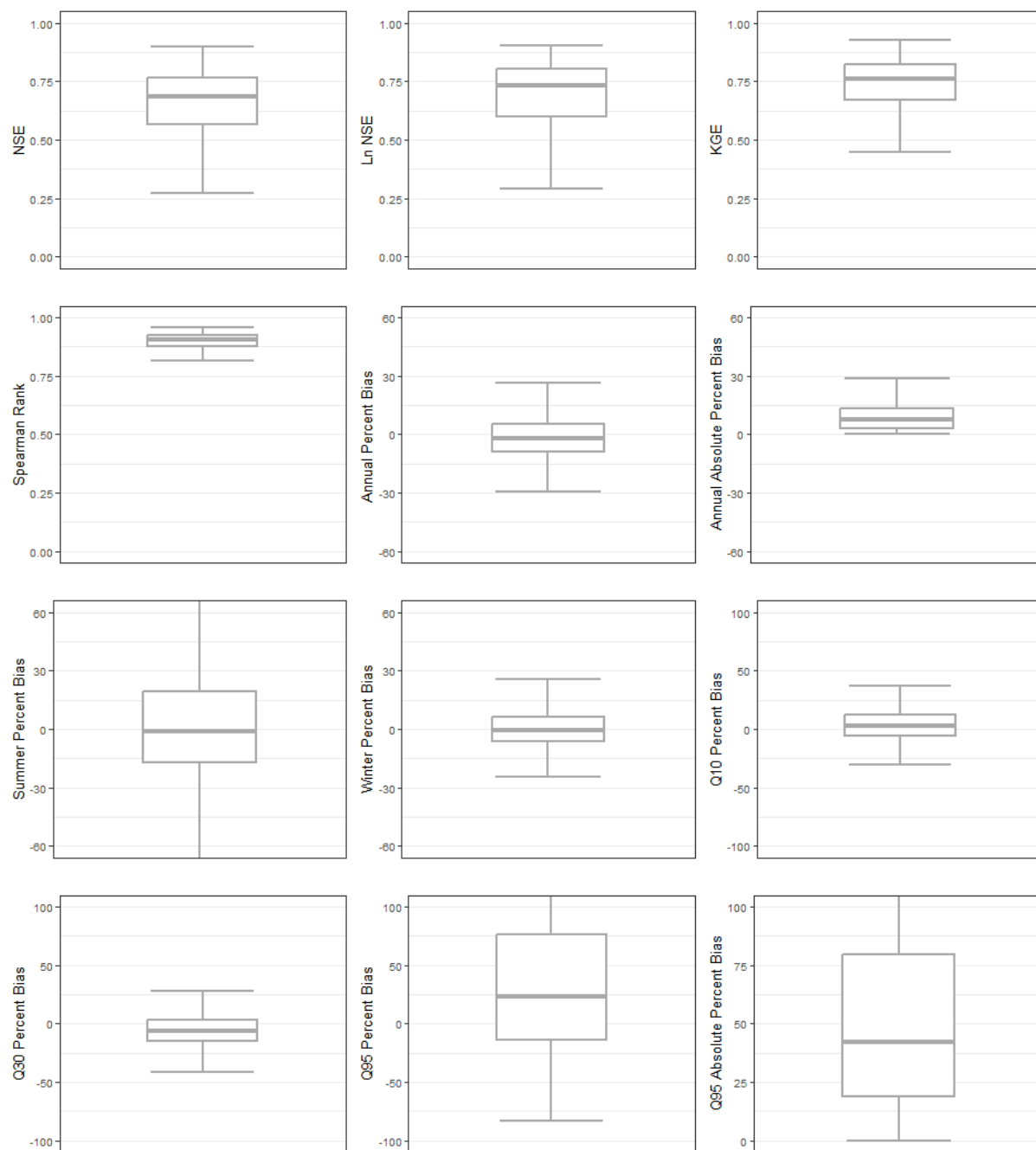
Figure 10. Box plots of the measures of fit for the CERF2 HadUK development dataset.
